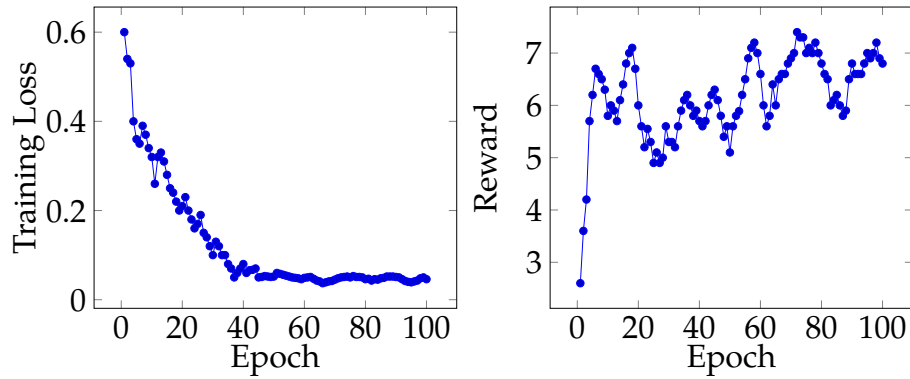
Figure 6.7: Training loss and rewards achieved by the RL policy.
